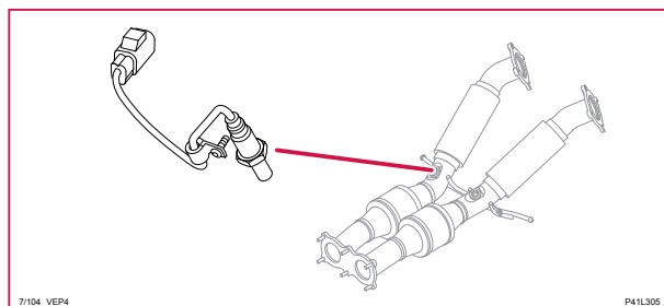
7/104 Bakre lambdasond
