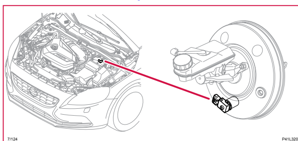
7/124 Givare bromspedal
