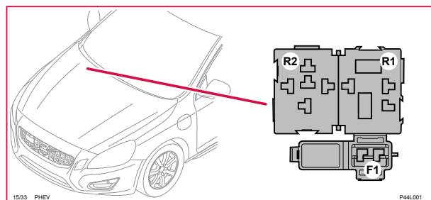
15/33 Elcentral, kall zon, motorrum
