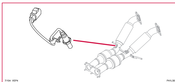
7/104 Bakre lambdasond, S60LH
