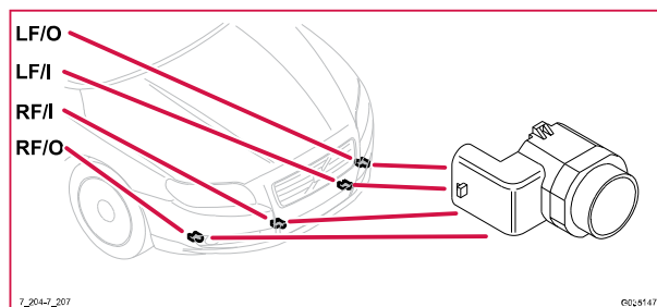
7/204-207 Sensorer parkeringsassistans fram
