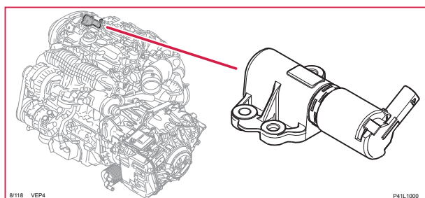
8/118 Solenoid variabel ventiltid, avgassida, S60LH
