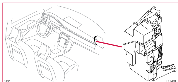
15/36 Elcentral, kupé
