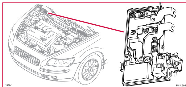
15/37 Elcentral, kall zon, motorrum
