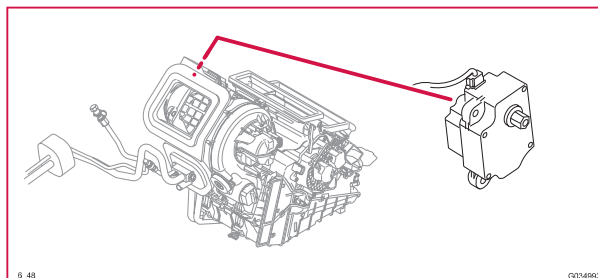
6/48 Styrenhet spjällmotor (DMM), recirkulation
