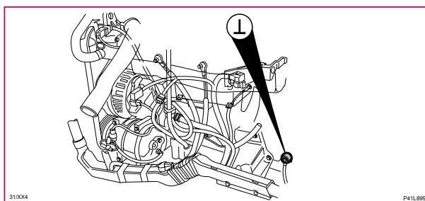
31/XX4 Stomanslutning, motor-kaross
