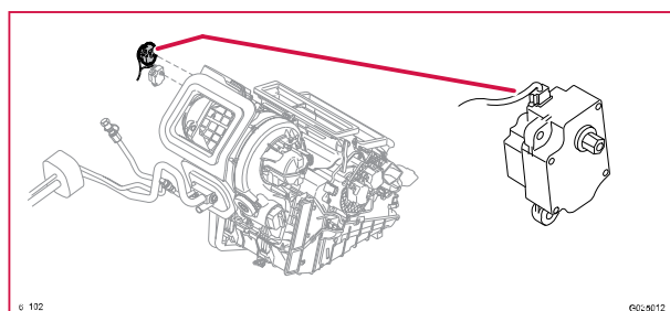
6/102 Styrenhet spjällmotor (DMM), defroster
