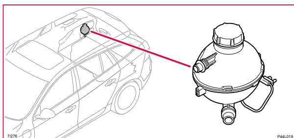
7/276 Nivågivare expansionstank
