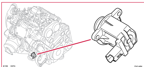
8/159 Bypass ventil
