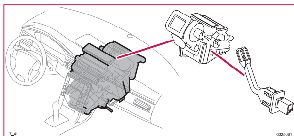
7/41 Temperatursensor, evaporator
