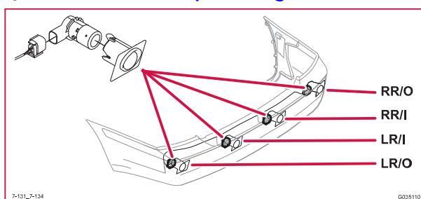
7/131-134 Sensorer parkeringsassistans bak
