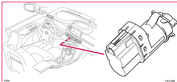
3/284 Diagnoskontakt bromsljus
