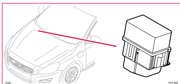
15/46 Reläcentral, motorrum
