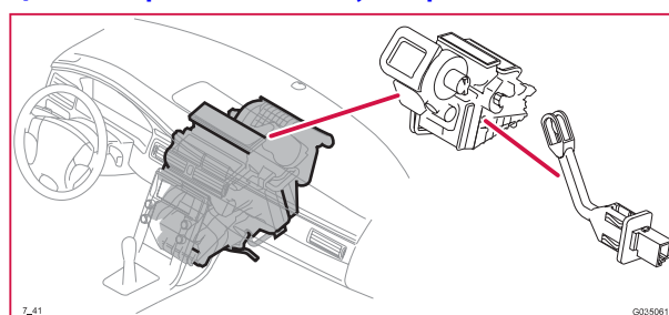
7/41 Temperatursensor, evaporator
