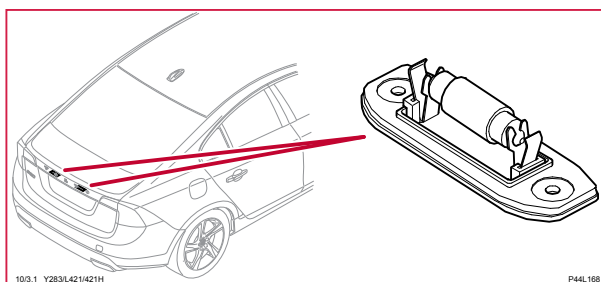
10/3 Skyltbelysning, S60LH
