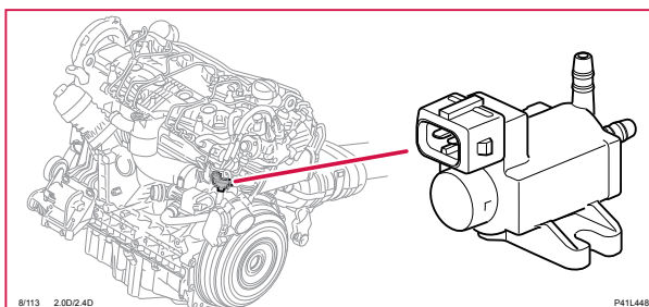
8/113 Bypassventil EGR-kyllning, V60H
