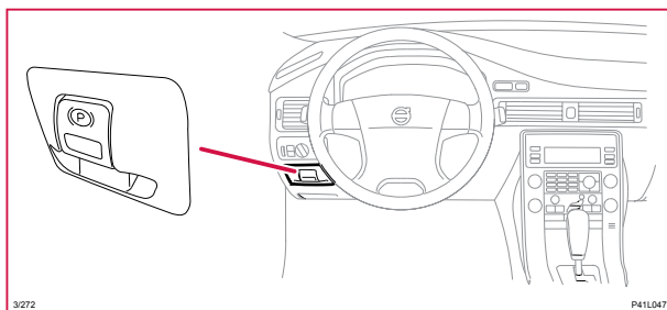
3/272 Omkopplare parkeringsbroms
