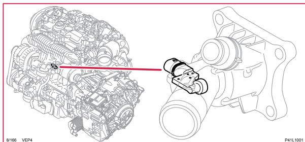
8/166 Elektrisk termostat, motorkylsystem, 4-CYL P
