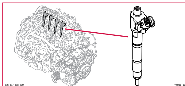
8/6-9 Insprutningsventil, 4-CYL
