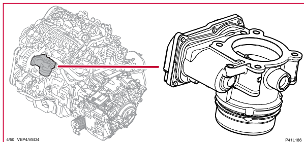
4/50 Gasspjällenhet, 4-CYL
