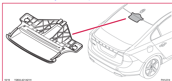
10/19 Bromslys extra, S60
