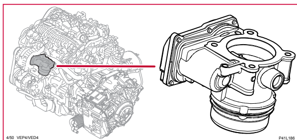
4/50 Gasspjällenhet, S60LH
