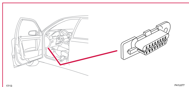
17/13 Diagnosuttag
