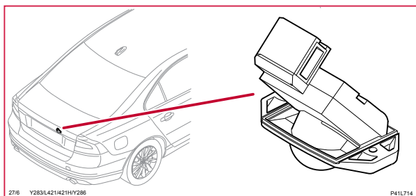
27/6 Kamera, S60LH
