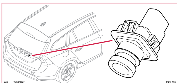
27/6 Kamera, V60H
