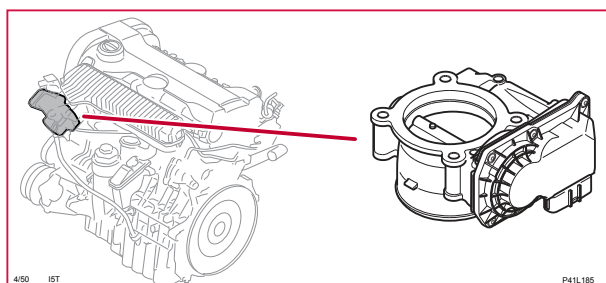
4/50 Gasspjällenhet, 5-CYL P
