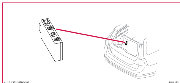
4/110 Styrenhet dragkrok (TRM), V60
