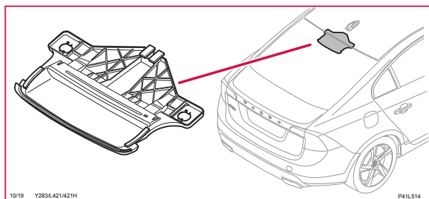
10/19 Bromsljus extra, S60
