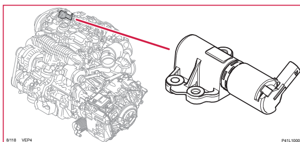
8/118 Solenoid variabel ventiltid, avgassida, 4-CYL P
