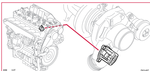
8/68 Luftbypass-ventil, 6-CYL
