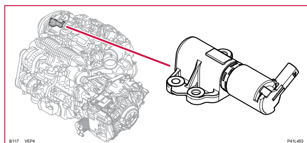
8/117 Solenoid variabel ventiltid, insugssida, 4-CYL P
