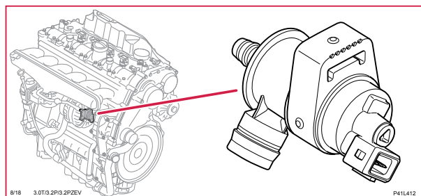
8/18 EVAP-ventil, 6-CYL
