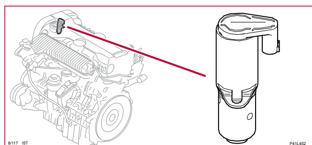
8/117 Solenoid variabel ventiltid, insugssida, 5-CYL P
