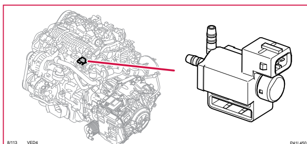
8/113 Bypassventil EGR-kylning, 4-CYL D
