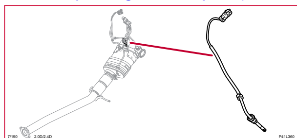
7/190 Temperaturgivare katalysator, 5-CYL D
