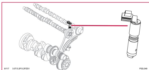
8/117 Solenoid variabel ventiltid, insugssida, 6-CYL
