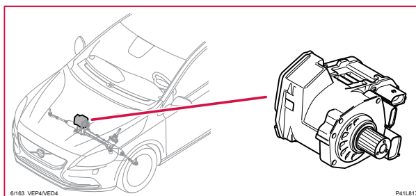
6/163 Elektrisk styrservo enhet (PSCM), 4-CYL
