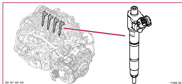
8/6-9 Insprutningsventil, 4-CYL
