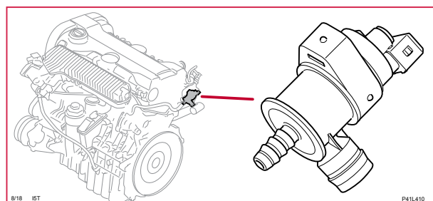
8/18 EVAP-ventil, 5-CYL P
