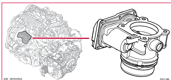
4/50 Gasspjällenhet, 4-CYL
