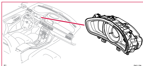
5/1 Kombinationsinstrument (DIM)
