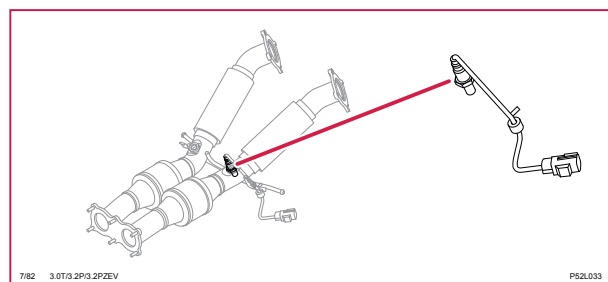
7/82 Bakre lambdasond, bank 1, 6-CYL
