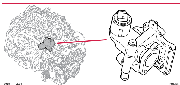
8/120 EGR-ventil, 4-CYL D
