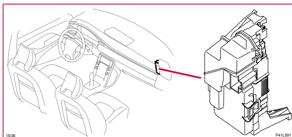
15/36 Elcentral, kupé
