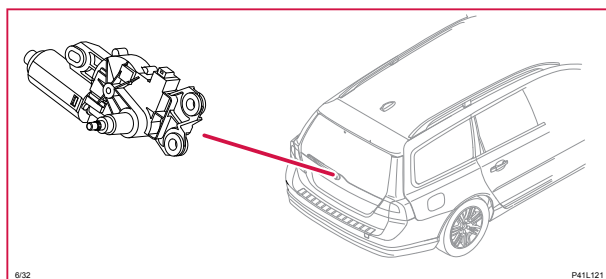
6/32 Motor bakrutetorkare
