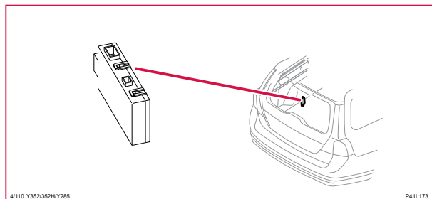
4/110 Styrenhet dragkrok (TRM), V70, XC70
