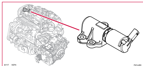
8/117 Solenoid variabel ventiltid, insugssida, 4-CYL 2.0P
