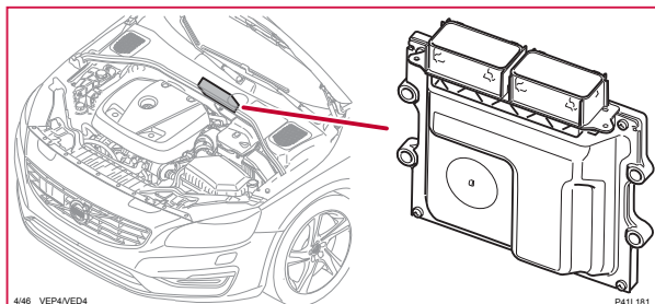
4/46 Styrenhet motor (ECM), 4-CYL 2.0L
