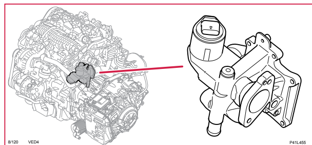
8/120 EGR-ventil, 4-CYL 2.0D
