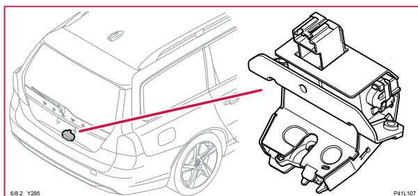
6/8 Centrallåsmotor, bagageutrymme, V70, XC70
