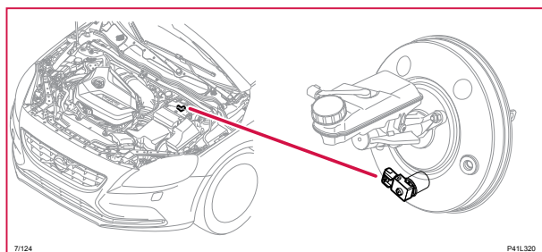
7/124 Givare bromspedal
