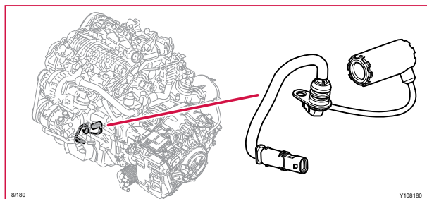
8/180 Motoroljepump solenoid
