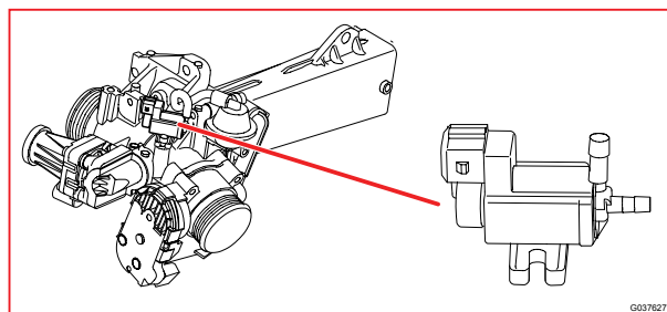
8/113 Bypassventil EGR-kylning, 5-CYL DIESEL
