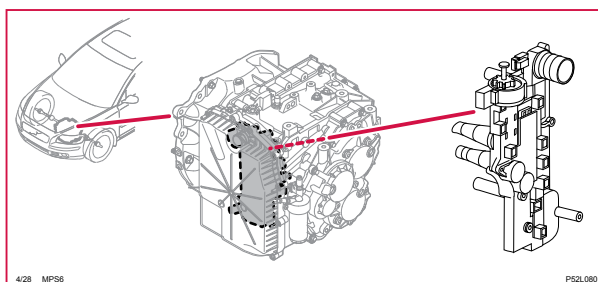
4/28 Styrenhet transmission (TCM), MPS6
