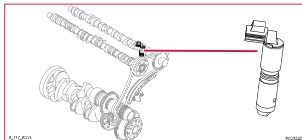
8/117 Solenoid variabel ventiltid, insuggsida, 6-CYL
