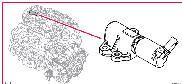
8/117 Solenoid variabel ventiltid, insuggsida, 4-CYL
