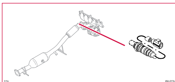
7/15 Främre lambdasond, 4-CYL
