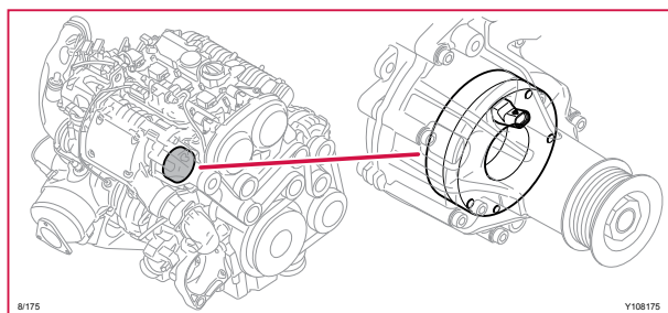
8/175 Kompressorkoppling, 4-CYL
