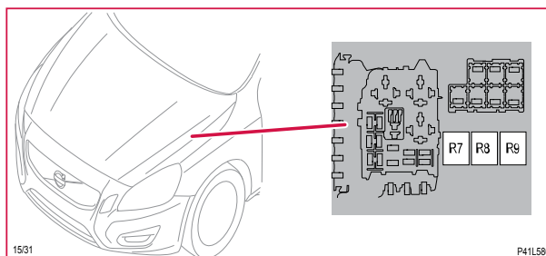
15/31 Elcentral motorrum
