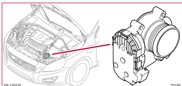
4/50 Gasspjällenhet, DIESEL
