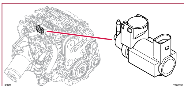
8/199 Vakuumpregulator, turbo bypassreglering
