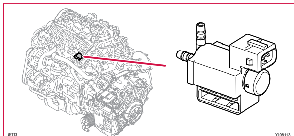
8/113 Bypassventil EGR-kylning, 4-CYL DIESEL
